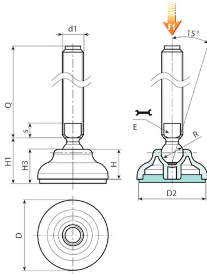
Version P910: Mounting foot with stem type B (with milled seat for wrench) and ball 15 - with SBS non-slip base
