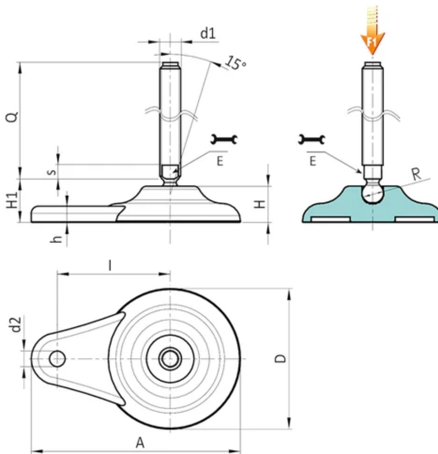
Version P706: Teardrop mounting foot with ground fixing - stem type B (with milled seat for wrench) and ball 15
